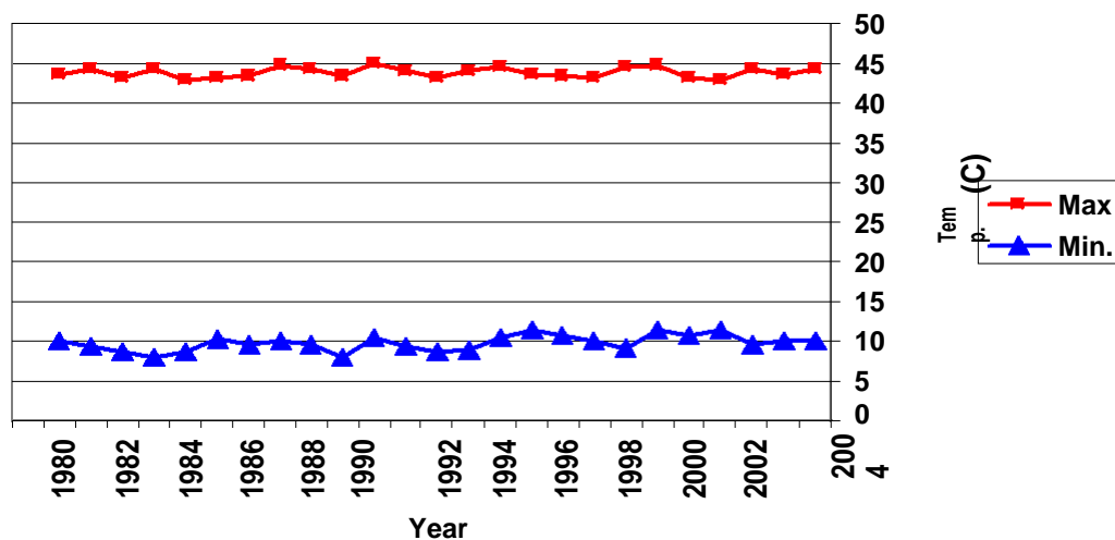
Figure 2. Average maximum and minimum temperature (°C) of the Sultanate of Oman for the years 1980-2004 (Source: Ministry of National Economy, Statistical Year Book 2005).
