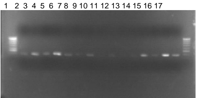
Figure 2. Multiplex PCR of DNA extracted from 14 field isolates of C. perfringens isolates in addition to a reference strain of C. perfringens type A. Lanes 1 and 17, 100-bp DNA molecular marker; lanes 2 through 15, C. perfringens field isolates; lane 16, C. perfringens type A reference strain. A single PCR-amplified DNA band, corresponding in size to the alpha ( ) toxin-encoding gene (approximately 402 bp), can be visualized on the agarose gel.
