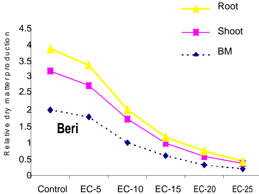
Figure 1. Relative dry matter production of browseable material, shoot and root as affected by salinity.
