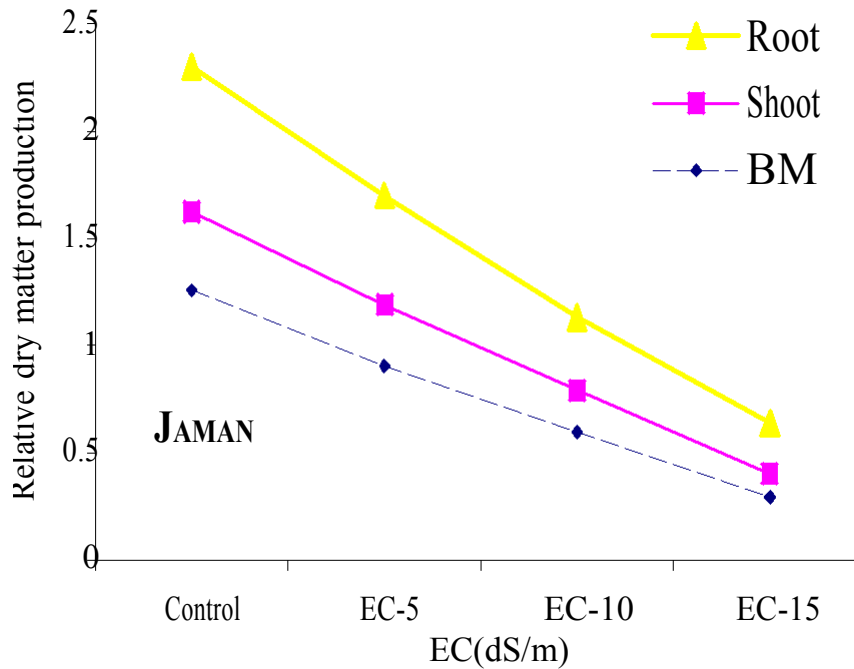
Figure 2. Relative dry matter production of browseable material, shoot and root as affected by salinity.
