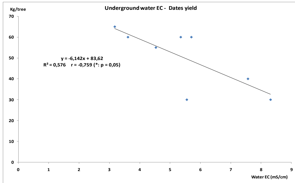
Figure 4. Correlation straight line between the underground water salinity and yield of palm trees.
