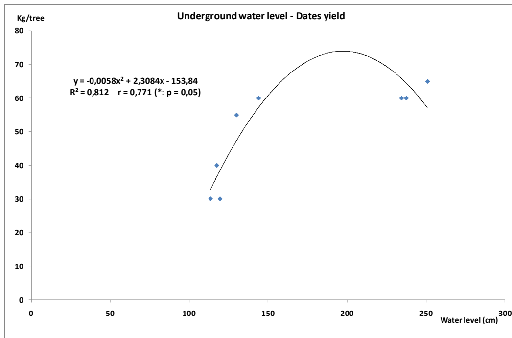
Figure 3. Correlation curve between the underground water level and yield of palm trees.
