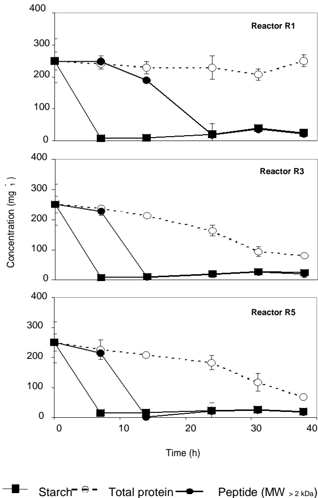
Figure 1. Kinetics of starch and BSA removal by A. niger under transitory conditions in reactors R 1 , R 3 and R 5 . Average initial synthetic wastewater composition: Starch, 250 mg l -1 ; BSA, 260 mg l -1 . Initial biomass concentration in the reactor R 1 was 1185 mg l -1 .
