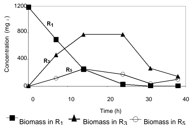
Figure 2. Kinetics of A. niger biomass migration through the reactors R 1 , R 3 et R 5 . Initial biomass concentration in the reactor R 1 was 1185 mg l -1 .
